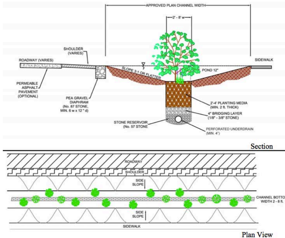
Figure 4.6 Bio-swale Plan and Section View (MDE, 2009)
