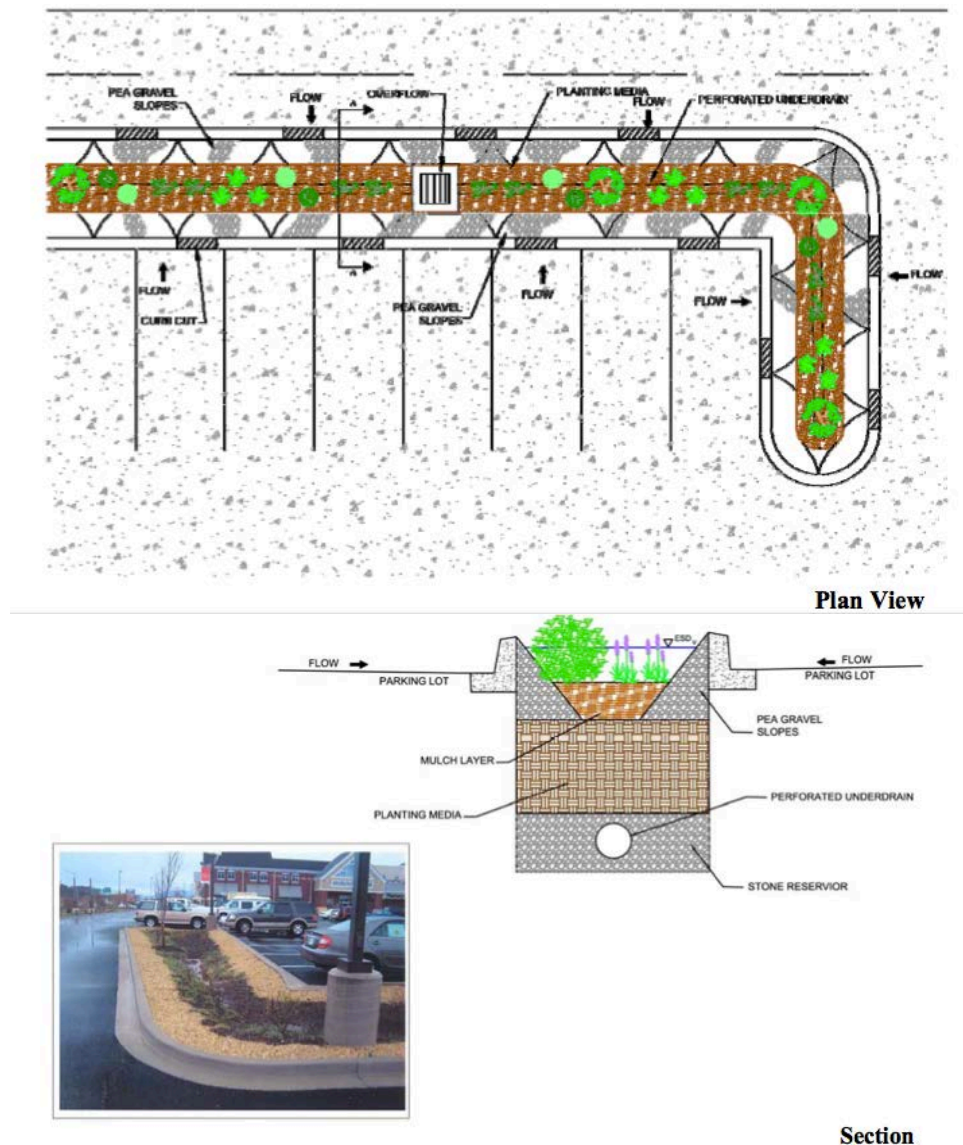
Figure 4.9 Micro-bioretention Plan and Section View (MDE, 2009)
