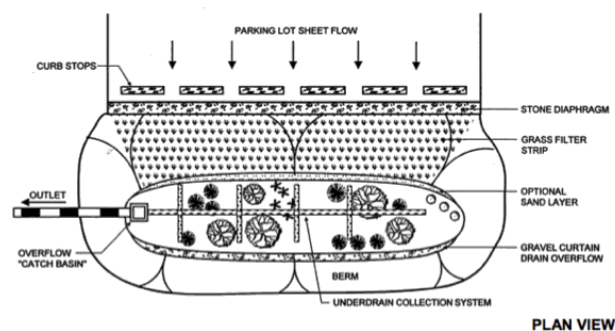
Figure 4.1 Bioretention Plan and Section View (MDE, 2009)
